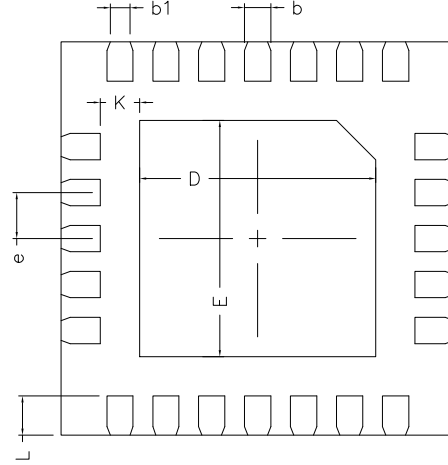
BOTTEM VIEW
