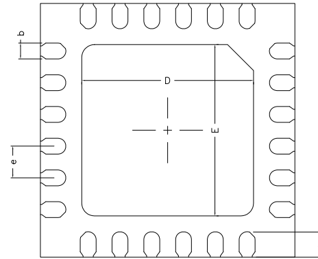
BOTTEM VIEW
