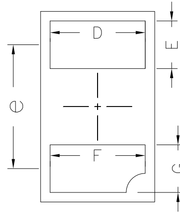
BOTTEM VIEW
